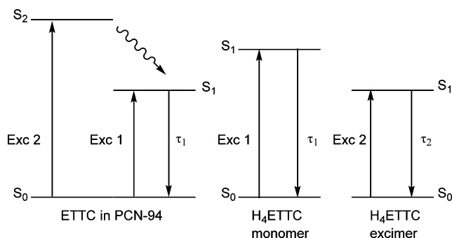
Figure 5. Schematic representation of the electronic transition levels of ETTC in PCN-94 and H_4ETTC .
